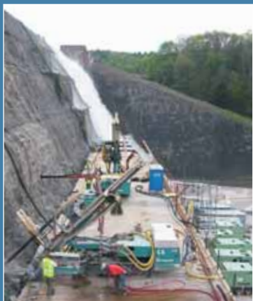
Anchor installation in Gilboa Dam spillway
