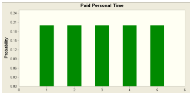
Figure 6. Personal days: 1 through 5 with equal probabilities
